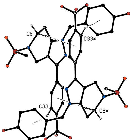
Figure 5 Part of the crystal structure of compound (I), showing the formation of a centrosymmetric dimer. For the sake of clarity, the unit-cell outline and H atoms bonded to C atoms not involved in the motif shown have been omitted. Atoms marked with an asterisk (*) are at the symmetry position (-x + 1, -y + 1, -z + 1) .
