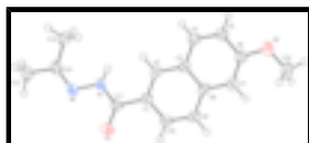
Fig. 1. Perspective view of the title compound with the atom numbering; displacement ellipsoids are at the 50% probability level.
