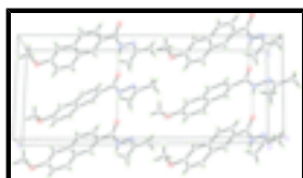
Fig. 2. Packing diagram of the title compound; hydrogen bonds are shown as dashed lines.
