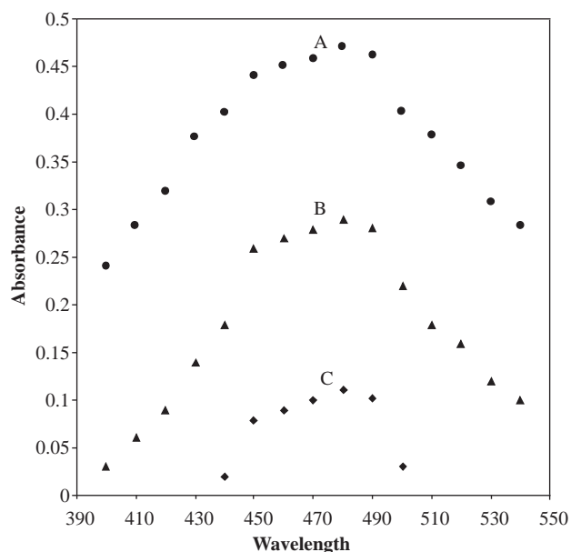
Figure 2. Absorption Spectra of: A. Blank containing 250 µg Ce(IV) sulphate in 10 ml B. and C. Reaction mixture of 250 µg Ce(IV) sulphate after treatment with 20 µg and 40 µg of PPH, respectively, in 10 ml.
