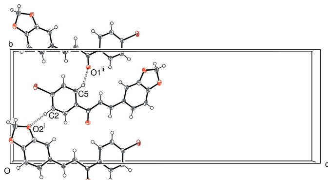
Figure 2 A fragment of the packing of (I), with the C—H...O interactions shown as dashed lines (symmetry codes as in Table 1).
