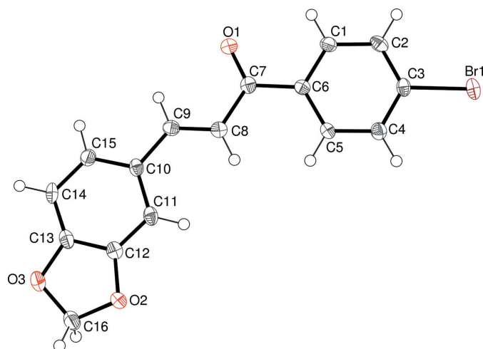
Figure 1 A view of the molecular structure of (I), showing 50% probability displacement ellipsoids (arbitrary spheres for H atoms).
