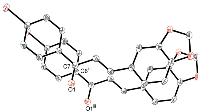
Figure 3 A fragment of the packing of (I), with the drawing projected on to the best plane of the O1 molecule, showing the offset of the aromatic rings of adjacent molecules stacked in the [100] direction. H atoms have been omitted for clarity. The closest intermolecular contact is 3.460 (5) Å for C7...C6 iii . [Symmetry code: (iii) x - 1, y, z .]
