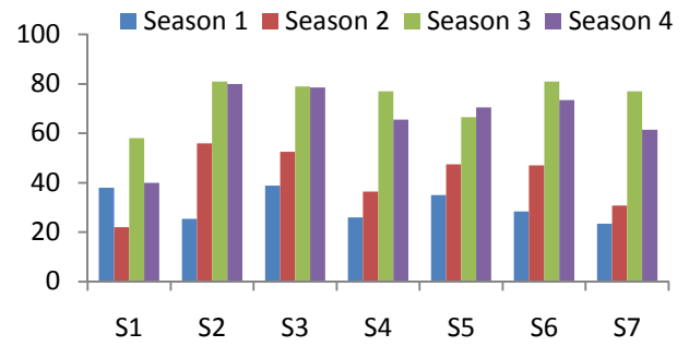
Fig.- 2l. Chloride (mg/L)
