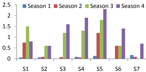
Fig. -2m. Phosphate (mg/L)
