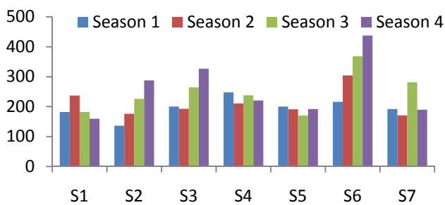
Fig. -2g. Total hardness (mg/L)
