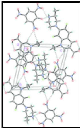
Fig. 2. Packing diagram of the title compound viewed down the a axis. Dashed lines indicate N—H···O hydrogen bonds creating a 2-D network along [011].
