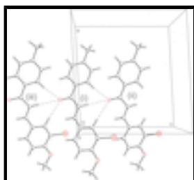
Fig. 2. The hydrogen - bonded chain of molecules of I . Hydrogen bonds are shown as dashed lines. Symmetry codes: (i) x, y, z ; (ii) x, 1/2-y, 1/2+z ; (iii) x, 1/2-y, -1/2+z .
