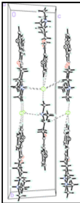
Fig. 2. Packing diagram of the title compound viewed down the a axis. Dashed lines indicate weak N—H...Cl and C—H...Cl intermolecular interactions forming a 2-D supramolecular layer which stacks along the b axis.
