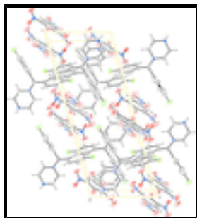
Fig. 3. Molecular packing of the title compound, viewed along [0\ 1\ 0] (anisotropic displacement ellipsoids drawn at 50% probability level).
